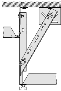
BULKHEAD TYPE 1B
