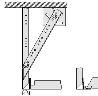
BULKHEAD TYPE 2A
